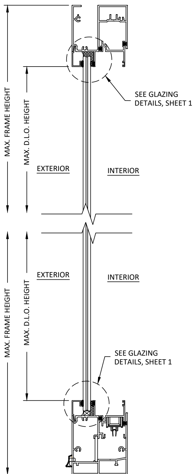
C 5 VERTICAL SECTION FIXED LITE DETAIL ALTERNATE WINDOW FRAME
