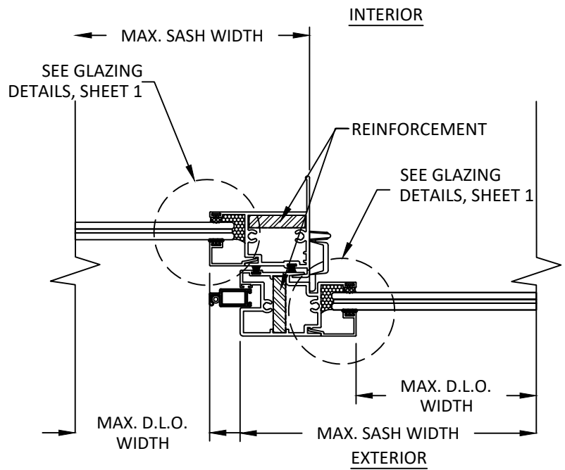
F 7 HORIZONTAL SECTION HEAVY REINFORCEMENT - MEETING RAIL
